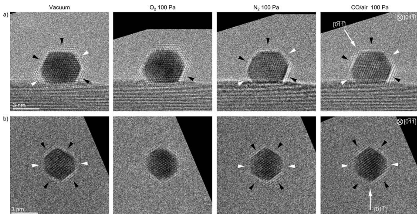
Figure 1. GNPs supported on TiO 2 . a) Lateral view of a GNP and b) top view of a different GNP. The viewing directions are [01 \bar{1} ] in (a) and [0 \bar{1}\bar{1} ] in (b). Black and white arrow heads indicate {111}- and {100}-type facets, respectively. The environment was varied from vacuum to O 2 (100 Pa) to N 2 (100 Pa) and to 1 vol% CO in air (100 Pa). Samples underwent electron irradiation only for acquiring ETEM images with a small electron current density, \phi = 3.0 \text{ A cm}^{-2} .
